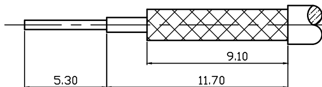
STRIP DIMENSION
