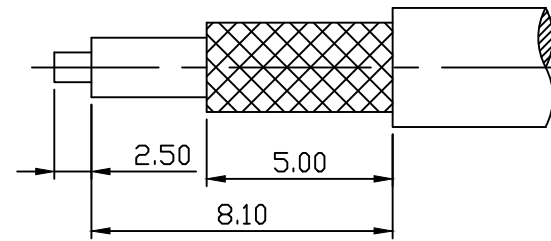
STRIP DIMENSION
