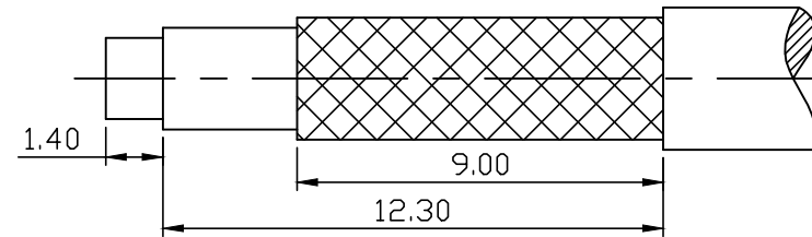
STRIP DIMENSION
