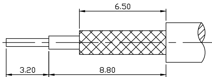
STRIP DIMENSION
