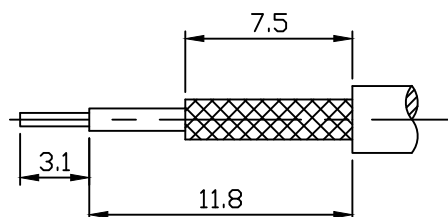
STRIP DIMENSION
